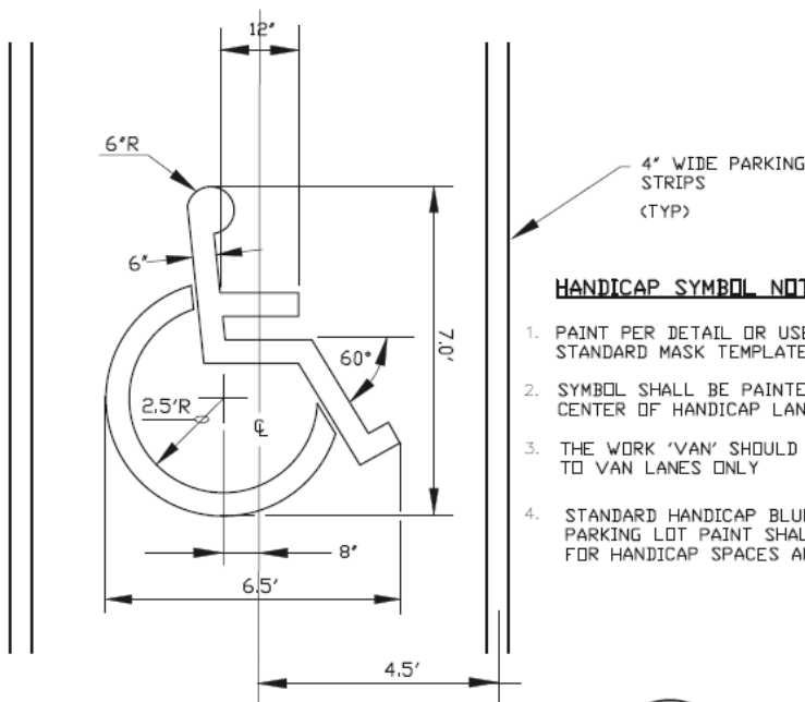
HANDICAP PARKING SYMBOL NOT TO SCALE
