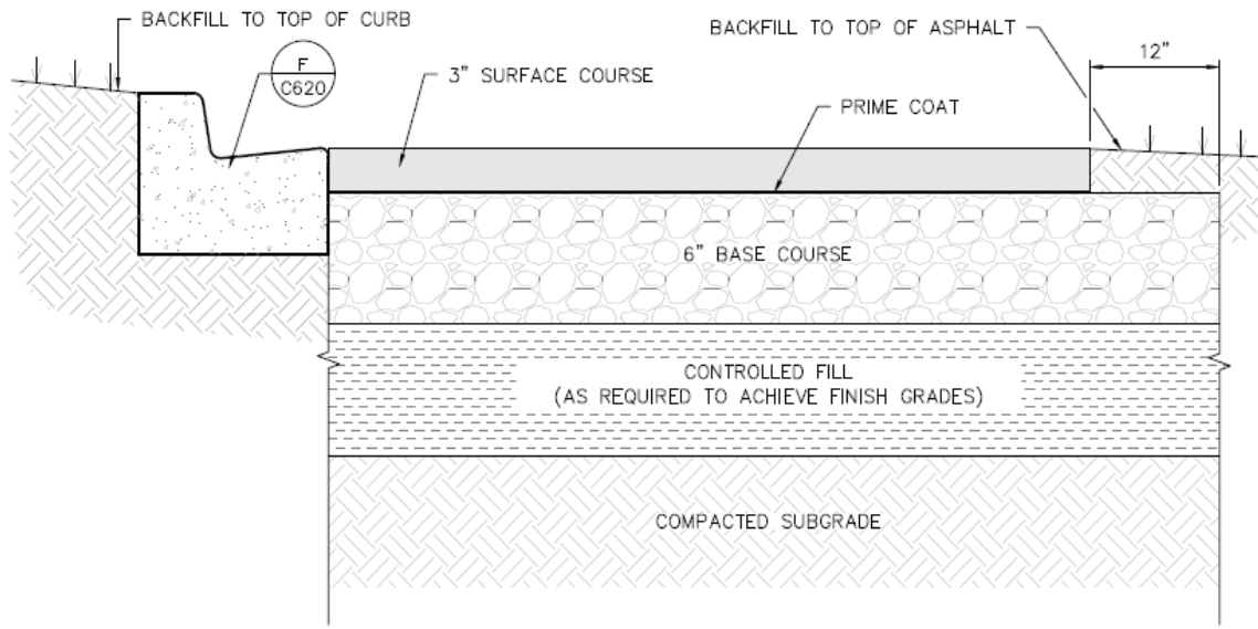
A STANDARD DUTY ASPHALTIC CONCRETE PAVEMENT SECTION
